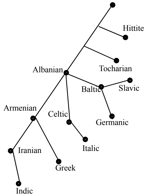
Minimal Spanning Tree (Hubey)
