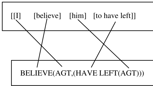
Figure 4 Possible RCG analysis of I believe him to have left
