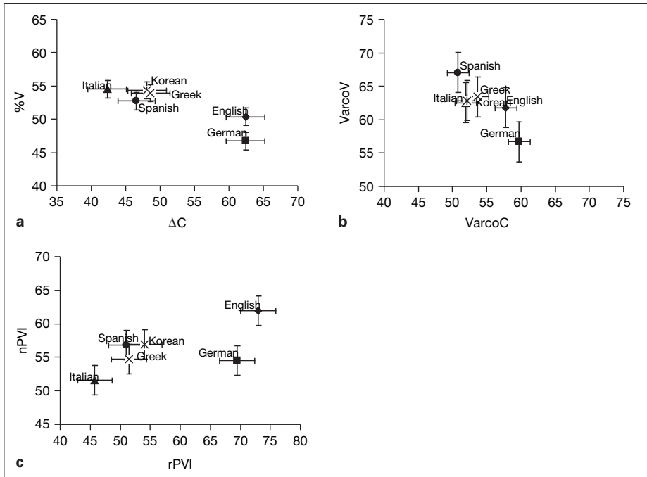
Fig. 5. a %V – \Delta C scores for English, German, Italian, Korean, Greek and Spanish calculated over the spontaneous speech data from the author’s study. b, c PVI and Varco scores for the same corpus.
